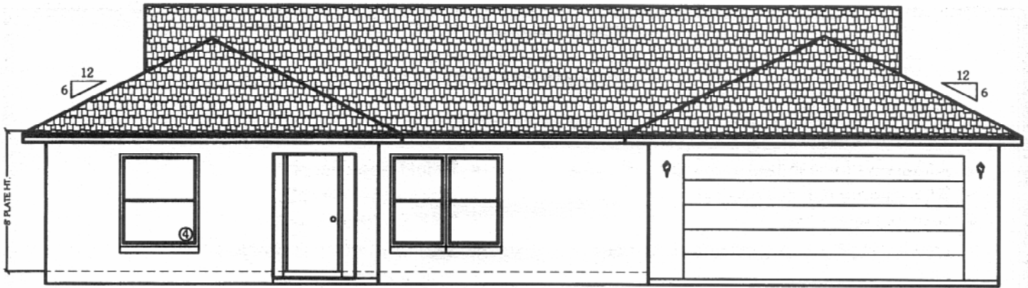
FRONT ELEVATION
